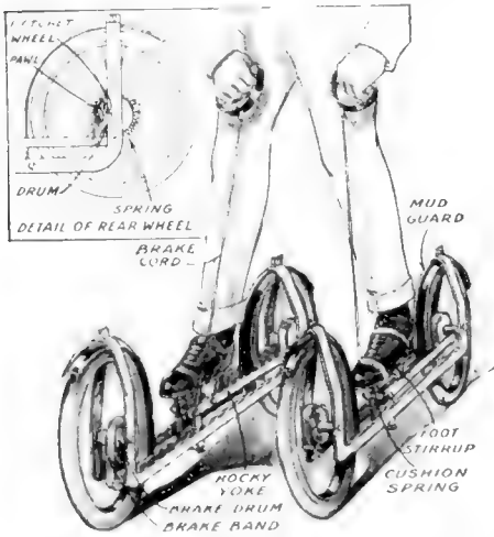
Fig. 4. Large wheels, a low center of gravity and a brake on the front wheel
